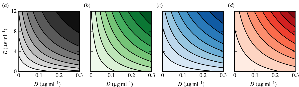
Figure 3. Contour plots of the drug inhibition surface \gamma(D, E) for different bacterial phenotypes (parameter values contained in table 1). Each line represents a 10% decrease of growth rate at a fixed concentration of resource ( S_0 = 2000 \mu\text{g ml}^{-1} ). (a) Susceptible phenotype, (b) E-resistant, (c) D-resistant and (d) multidrug, DE-resistant bacteria. (Online version in colour.)
