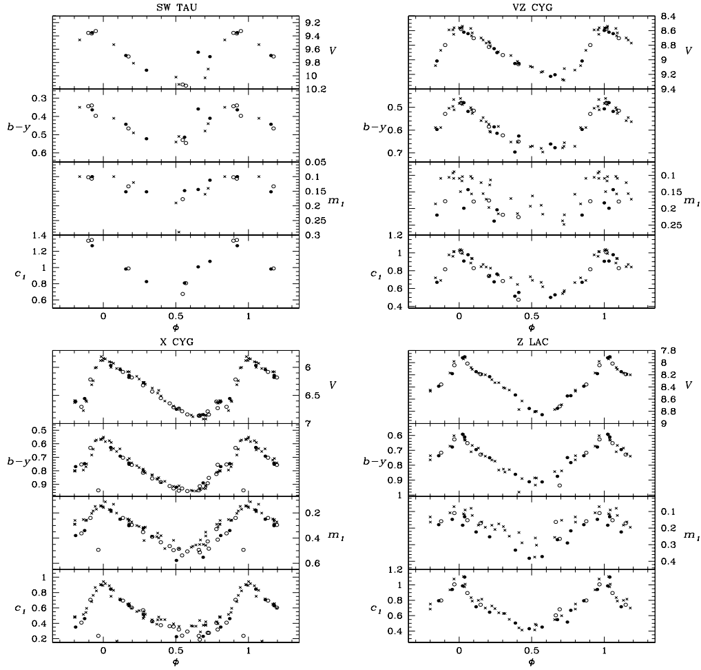
Fig. 2. Light curves in uvby - \beta for four stars observed by several authors. Note the good agreement between the various sources. Open circles: Arellano Ferro et al. (1998); crosses, Feltz & McNamara (1980); filled circles, present work.
