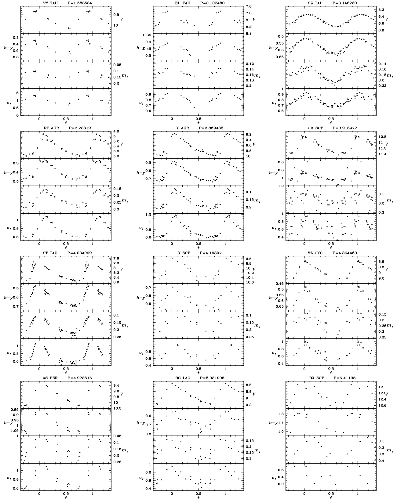
Fig. 3. uvby - \beta Light curves of program Cepheids.
